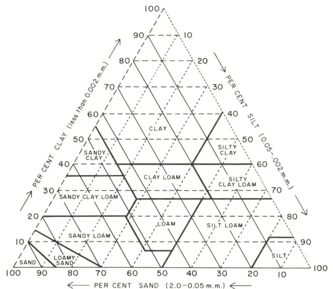
Fig. 1. The textural triangle, showing common soil textural classes.
