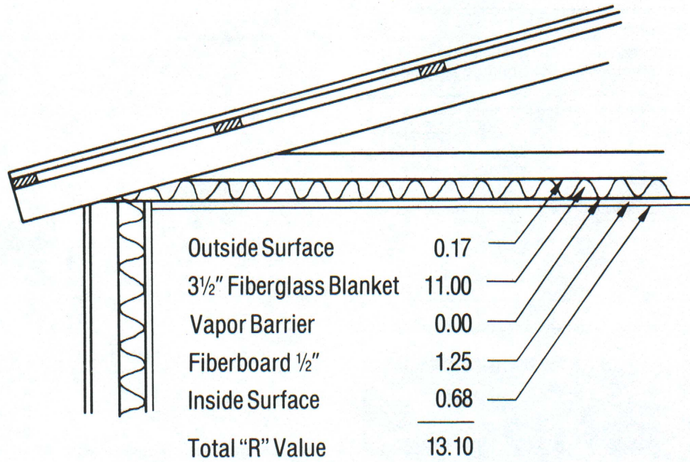
Figure 2. Insulated wood frame ceiling. Reducing the insulation to 1½ in. of fiberglass blanket reduces the ceiling R to 7. Using 6 in. of fiberglass insulation increases the ceiling R to 21.
