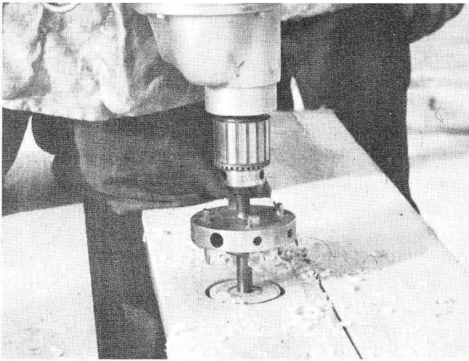
Fig. 3. A special grooving tool is used to cut a groove so split-ring connectors can fit halfway into each truss member. The tool fits in a half-inch electric drill. A 9/16-inch hole is first drilled in the member at the proper location so that it can be used as a guide in cutting the groove.
