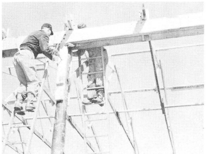
Fig. 19. The proper anchorage of the rafter supports, with scabs bolted in place, is important in pole frame buildings. All of the roof load is transferred to the sidewall poles in this case.
