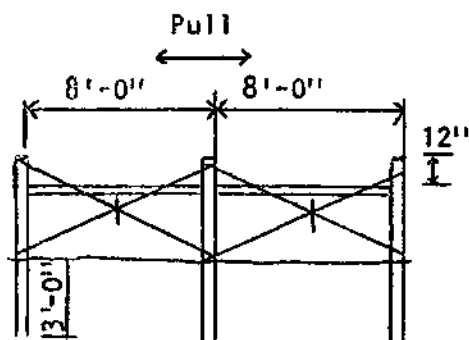
Fig. 2. Wood line pull brace. Use every 40 rods in long fences.
