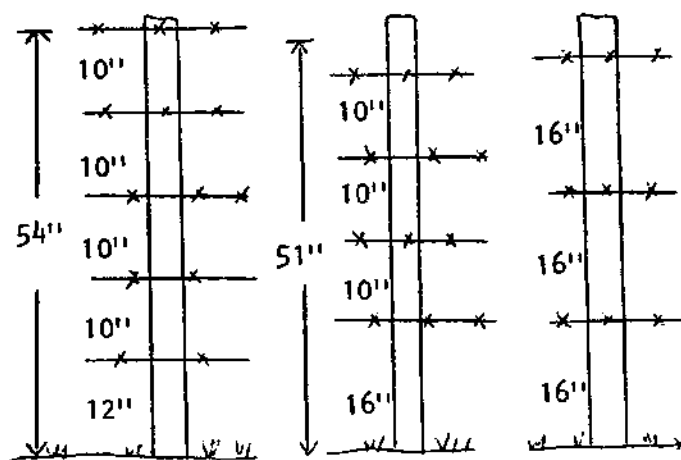
Fig. 3. Some typical barbed-wire spacings.
