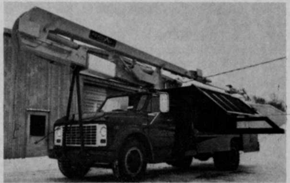
Hydraulically operated chip boxes, either side or end ejection.
