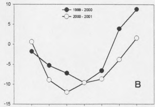
Change in minimum air temperature from October 1999 to April 2001
