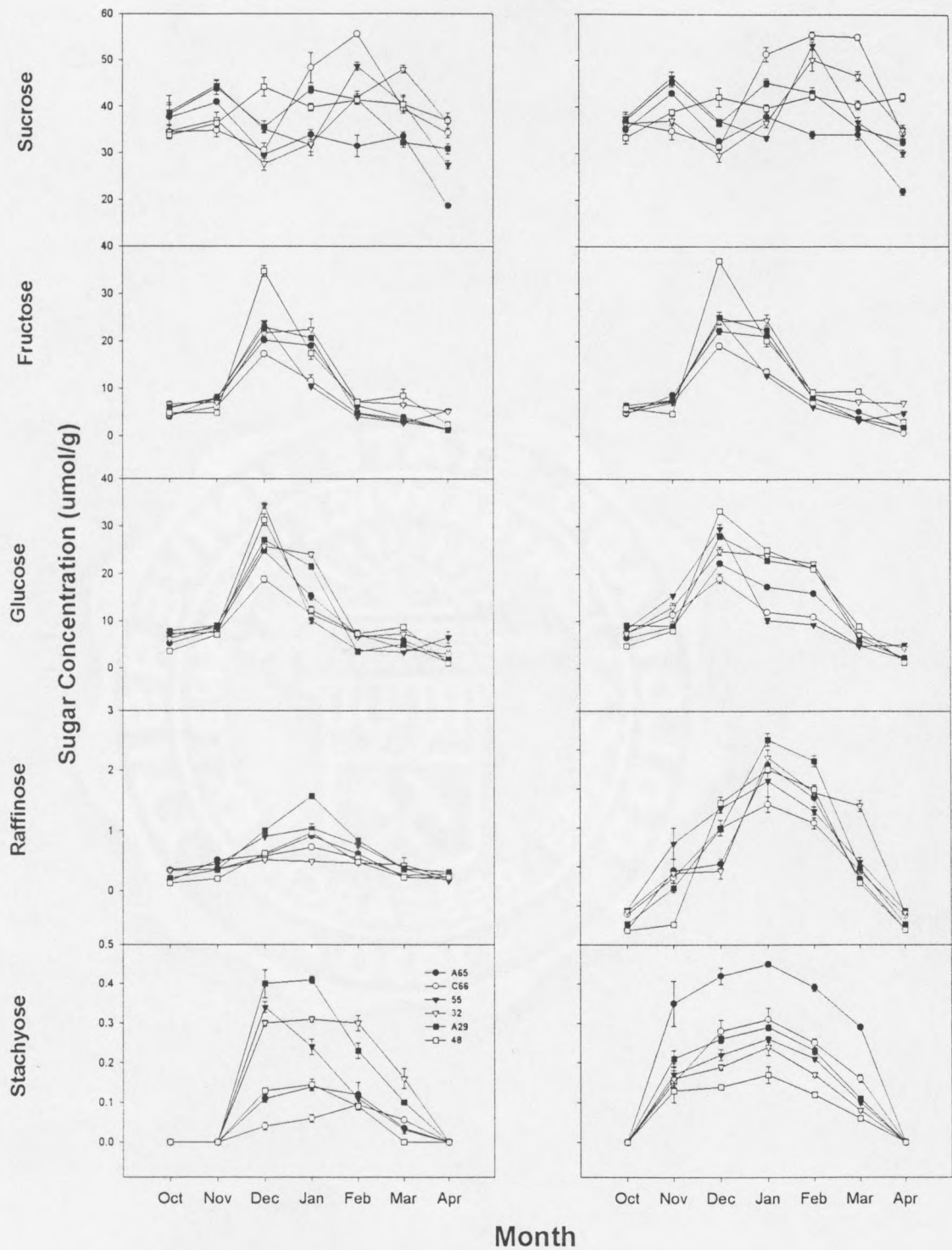
Fig. 2.3. Mean contents of sucrose, fructose, glucose, raffinose and stachyose of six saltgrass accessions tested from October 1999 to April 2000 (left panel) and from October 2000 to April 2001 (right panel). Bars represent the standard errors.
