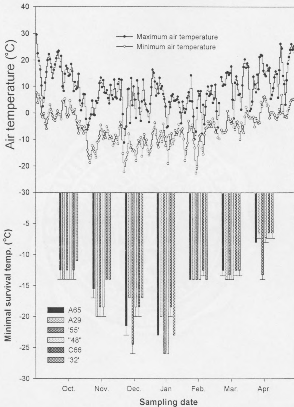
Fig. 2.2. Seasonal patterns of minimal survival temperatures of six saltgrass accessions sampled from Oct. 2000 to April 2001 in relation to the prevailing minimum and maximum air temperature at the sampling dates. Bars represent the standard errors.
