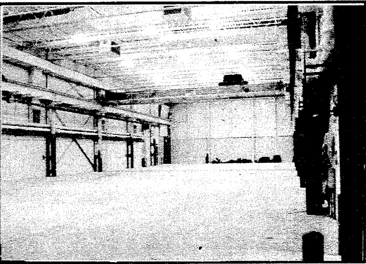
This picture shows the massive bays (3 at the south end of the building) where equipment is being set up for long term testing and research of both production equipment and product. Note the massive overhead crane that can position the equipment.
