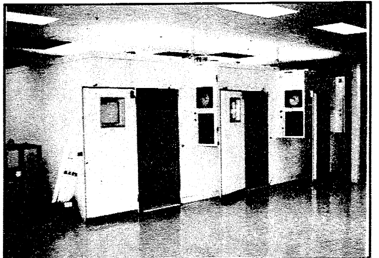
These three booths are equipped for temperature, pressure and climate controls to test the carbonation retention of plastic containers.
