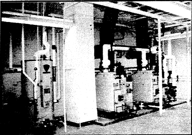
Two boilers and hot water heater, all in excess of 200,000 btu each, provide the heat and domestic hot water for the new facility.
