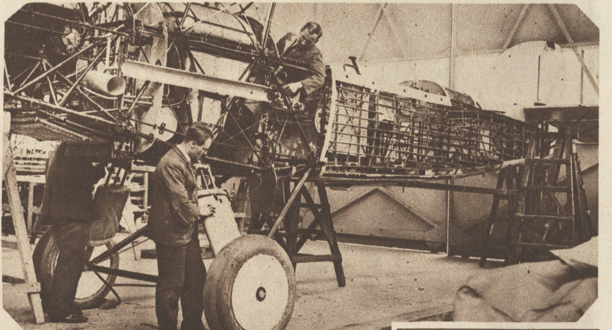
INTRICATE DETAIL of a modern fighting machine as revealed before the fuselage covering is put on. (© Acme photo.)
