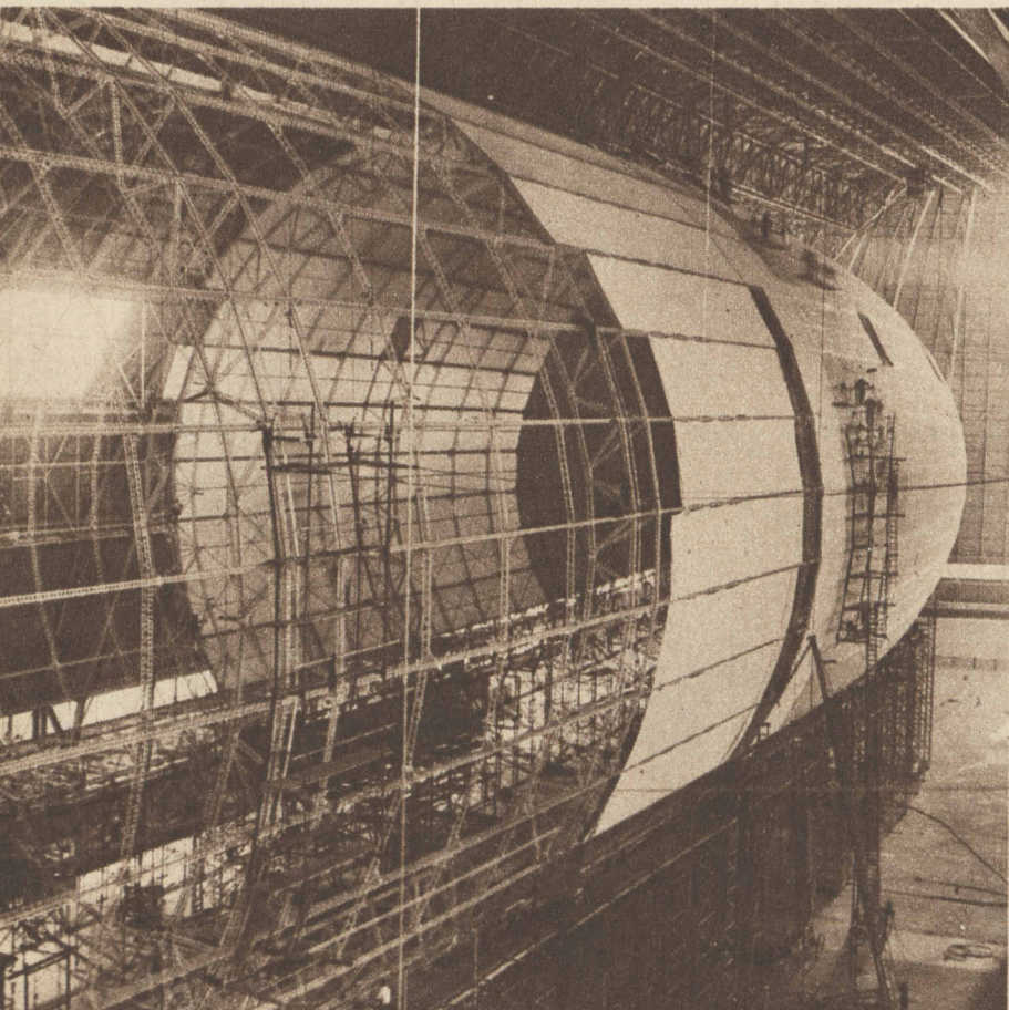
AMERICA'S AERIAL TAILORS fit the "skin" of the world's biggest dirigible, Akron, at Akron, Ohio. Note the size of the men as compared with the vast framework. (Associated Press photo.)
