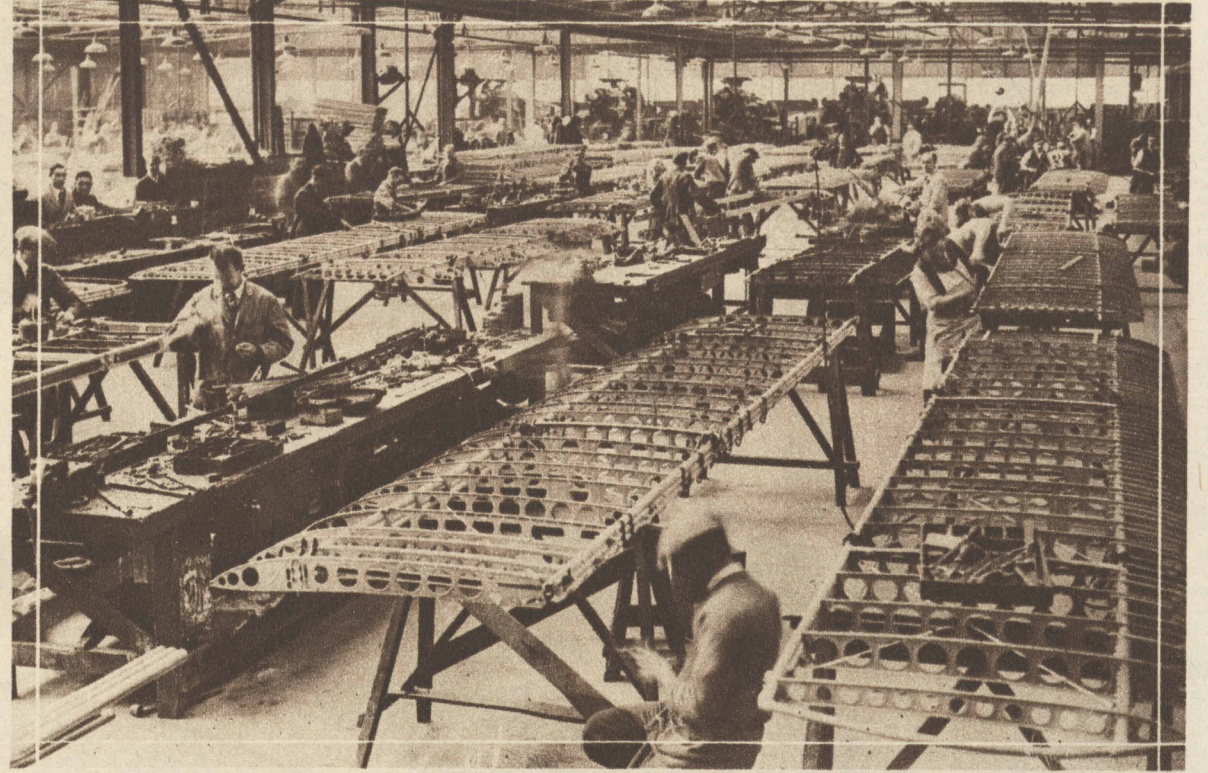
FOR ST. GEORGE AND MERRY ENGLAND—An imposing view of steel skeletons in the wing room, where precision instruments are employed in a vital part of plane fabrication. (© Acme photo.)
