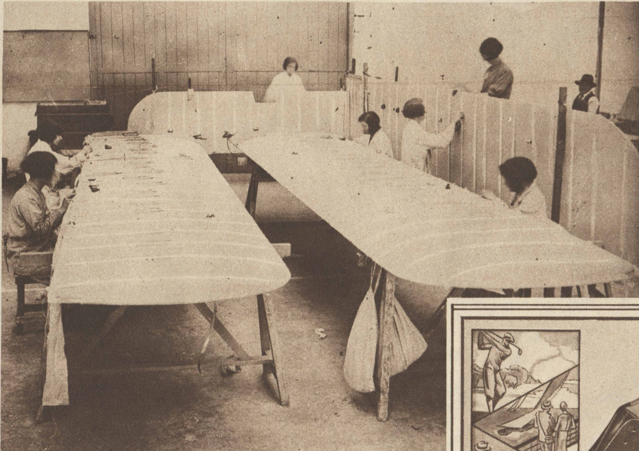
WOMAN COMES INTO HER OWN, in the manufacture of Britain's airplanes, in the delicate task of stitching the wing fabric. (© Acme photo.)
