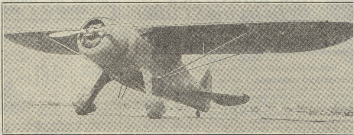
This new airplane, designed by Ben O. Howard, has a cruising speed of 198 miles an hour at 12,500 feet, with a maximum of 350 horsepower at takeoff and 205 horsepower while cruising. It carries four passengers and 120 pounds of baggage. Other similar planes have a cruising speed 50 to 70 miles slower. (Tribune Photo.)
