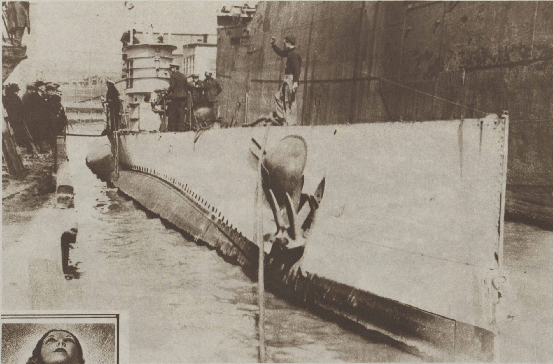
IN FOR REPAIR—A Peruvian submarine, the R-1, docks at Philadelphia. (Associated Press photo.)
