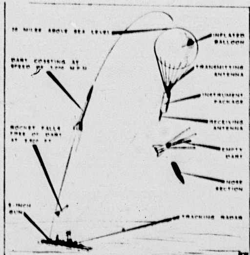
An anti-aircraft missile, found to be too small for its intended use, is what the Navy hopes to collect weather data with from altitudes as great as 50 miles high. It can be fired from the deck of a ship. Formerly the Tekt rocket, it is now called the HARP, nickname for the high altitude sounding projectile.
