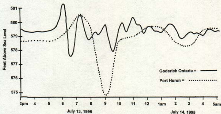
Figure 3. Sudden change in water level in southern Lake Huron on July 13, 1995, before, during and after a severe squall. Winds went from zero to 70 miles per hour in 30 minutes, with the storm front traveling approximately 50 to 60 miles per hour across the water. The lake oscillated for two days after this event.
