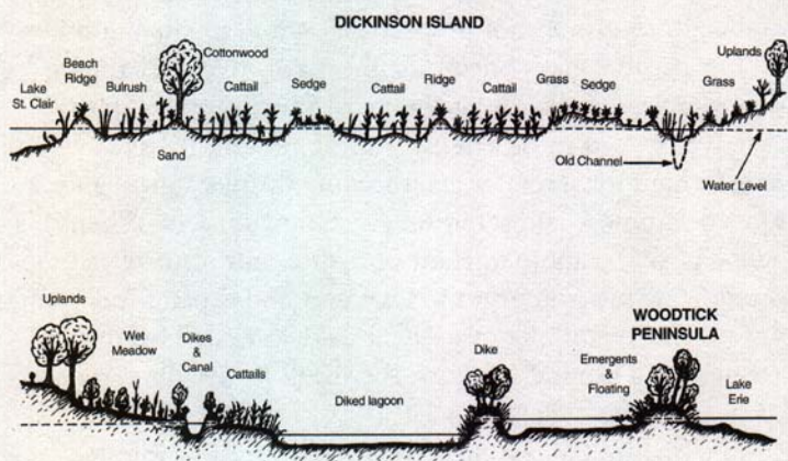
Figure 17. Dickinson Island (A) and Woodtick Peninsula (B) vegetation zones show a typical pattern for a delta wetland and a diked wetland. Note the deviation from classic zonation patterns shown by Dickinson Island, and water level lower than Lake Erie inside of Woodtick dike. See Figures 13 and 14.
