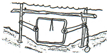
EXAMPLE OF LEG-HOLD TRAP SET FOR BEAVER
