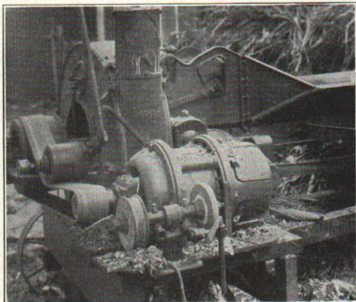
Five H. P. Electric Motor mounted on frame of cutter. Pulleys two feet apart at centers. Idler used on belt to give proper tension. Too tight a belt ruins the bearings of machinery.
