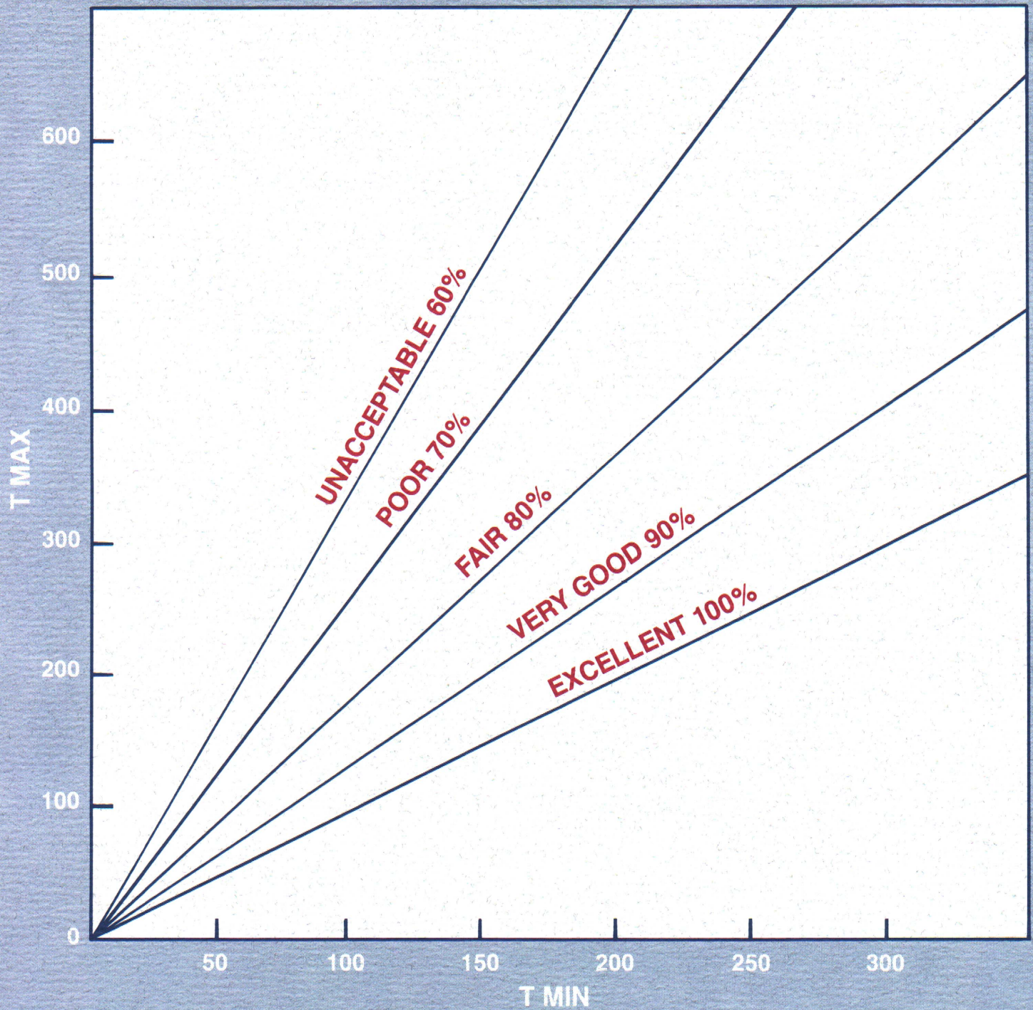
Figure 1. Field Method for Calculating System Uniformity
