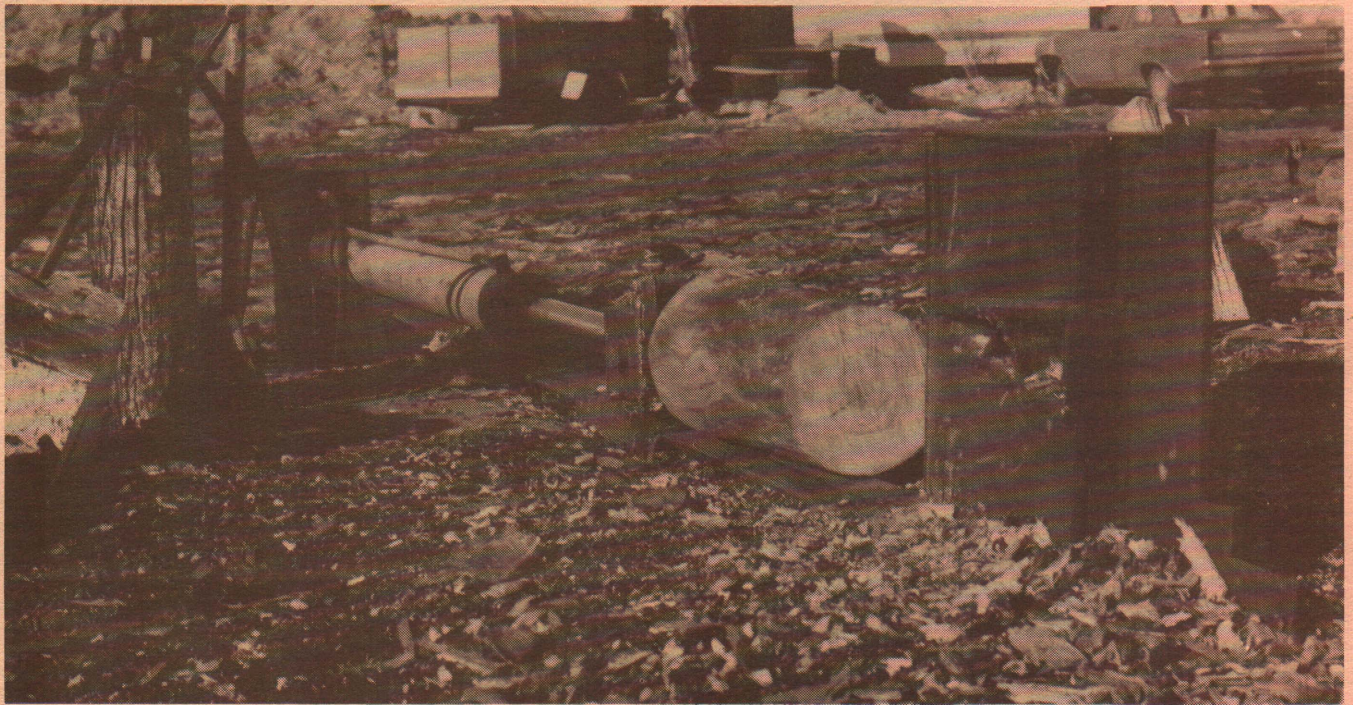
Figure 4. Where a large amount of wood is to be split, a power-operated splitting machine will reduce the amount of labor required while increasing the speed and ease of splitting. The hydraulic cylinder forces a block of wood against a stationary splitting wedge.
