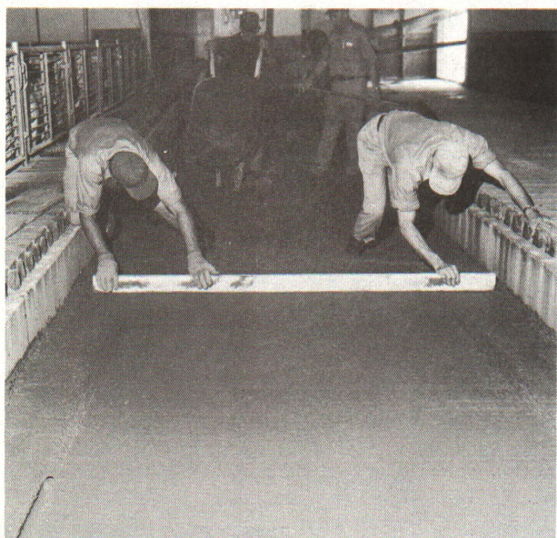
Fig. 6. Skirting concrete on two 1" pipes resting on the 2" x 4" stakes. Since the pipes have an outside diameter of 1\frac{1}{4} ", the length of the stakes must be reduced by this amount to give the desired floor elevation.
