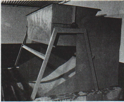
Fig. 2. Tanks can be mounted on a steel frame, poured concrete wall or a 6" concrete block wall. Likewise, the curved spillway can be constructed of concrete or metal. Use the material that fits your capabilities best.
