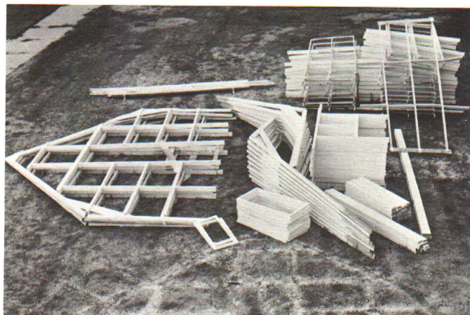
Fig. 2 Precut and prefabricated members for an 18 by 96 feet rigid frame greenhouse.
