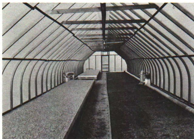
Fig. 8 Interior view of a laminated rafter greenhouse.
