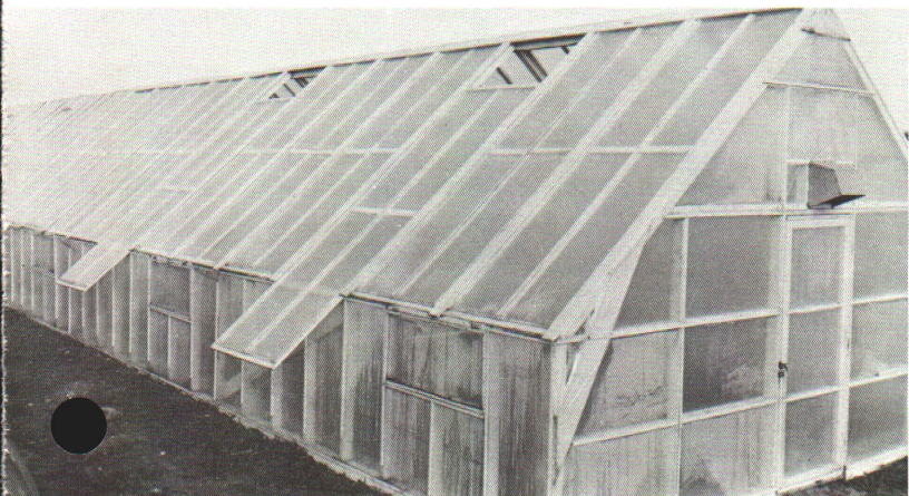
Fig. 6 Ridge ventilation in the panel house is accomplished by having sliding panels.
