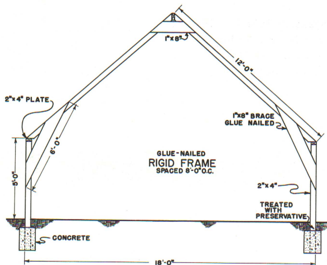
Fig. 1 Detail plan of the rigid frames which form the basic framework for the greenhouse.
