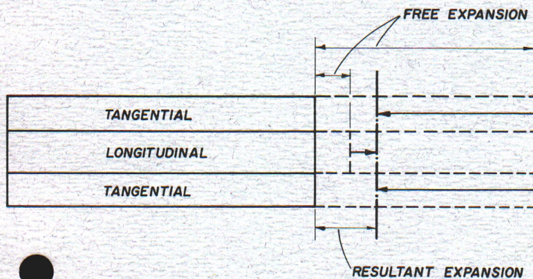
Figure 4. Resultant expansion of three-ply plywood.
