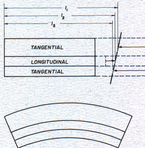
Figure 5. Warping of expanding three-ply panel due to unequal thickness of face and back veneers.
