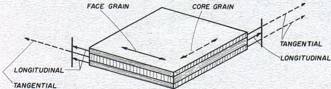
Figure 3. Mutual restraint of veneers in three-ply plywood.
