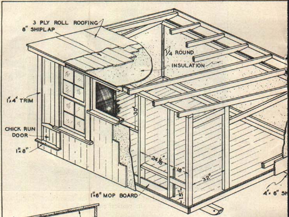
ISOMETRIC
