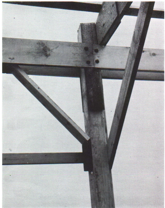
Figure 9—A well-constructed joint at the pole. Four bolts have been substituted for about one-half of the nails; wind braces in two directions.
