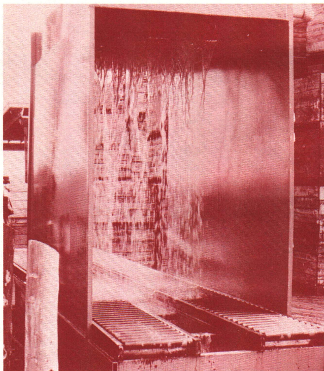
Fig. 2. Drench applicator suitable for applying calcium chloride to pallet bins of apples. A stack of two bins is placed onto the roller conveyor and pushed into the enclosed portion by a lift truck. The next stack of bins pushes the first stack to the back where it is removed after draining for a minute or so.
