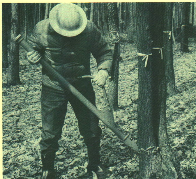
Figure 7 — Liquid herbicides can be applied by equipment which creates a frill and applies the herbicide in one simultaneous operation. The active ingredient being used at left is 2,4,5-T while cacodylic acid is being applied at right.
