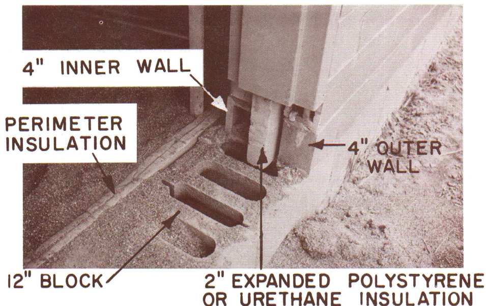
Fig. 2 With masonry construction, rigid insulation is used in a core wall. A special adhesive is used to seal the joints of the sheets of insulation to insure moisture resistance.
