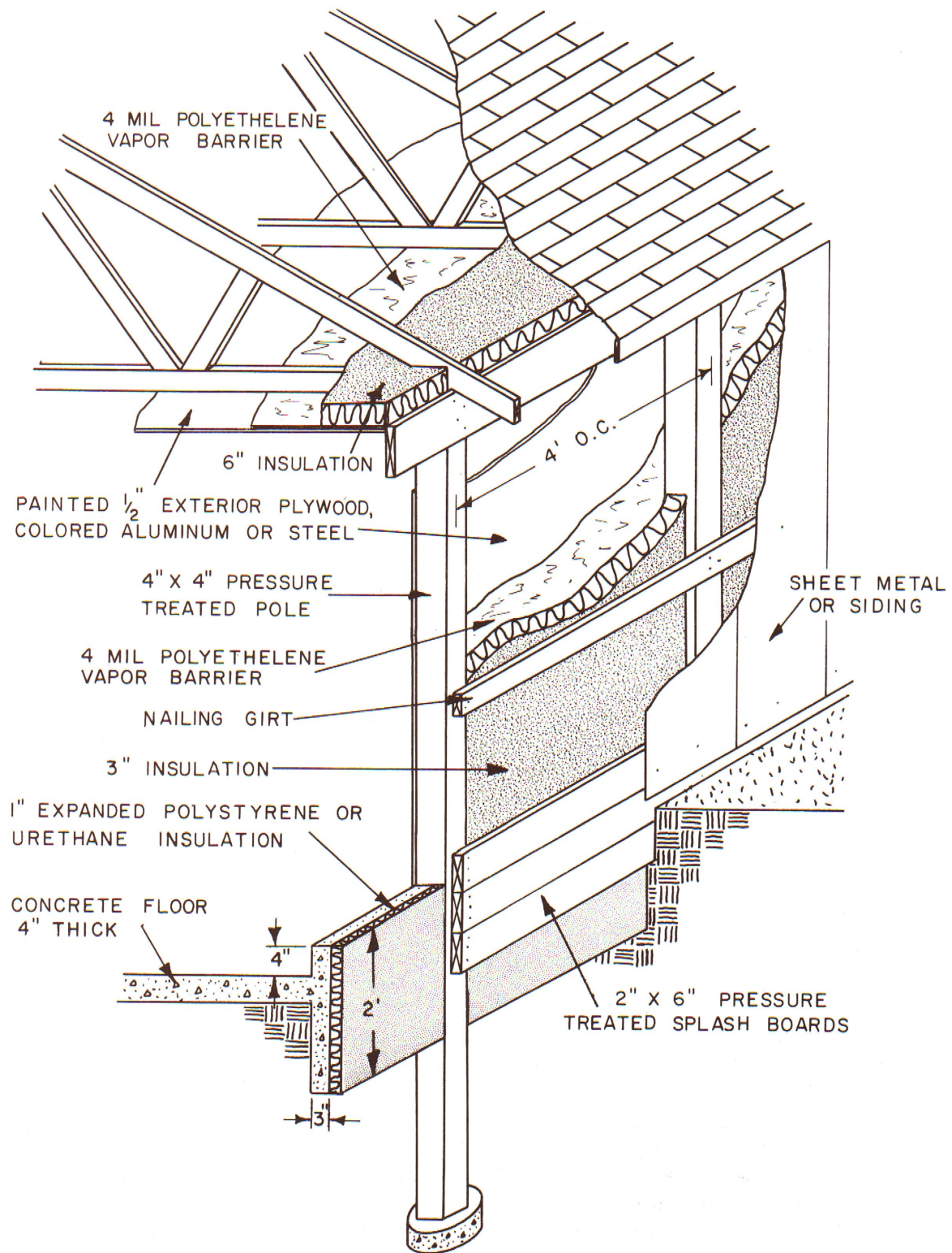
Fig. 1 This pole-frame wall has 4" x 4" pressure treated poles spaced 4 feet apart. A 4 foot wide roll of 3 inch blanket insulation is placed vertically in the spaces between the poles.
