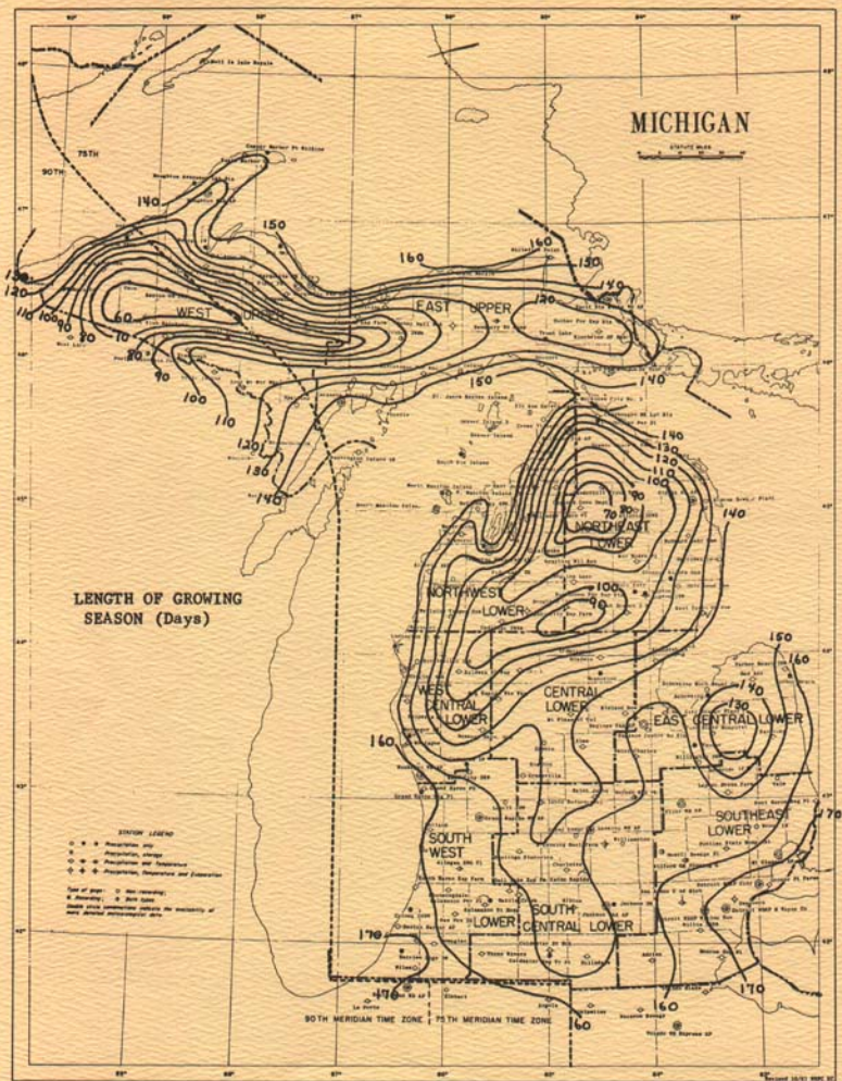
Fig. 1.—Length of growing season. The number of days between the average date of the last freezing temperature ( 32^{\circ} F or colder) in the spring to the average date of the first freezing temperature in the fall. (Data furnished by A. H. Eichmeier, U. S. Weather Bureau, East Lansing.)
