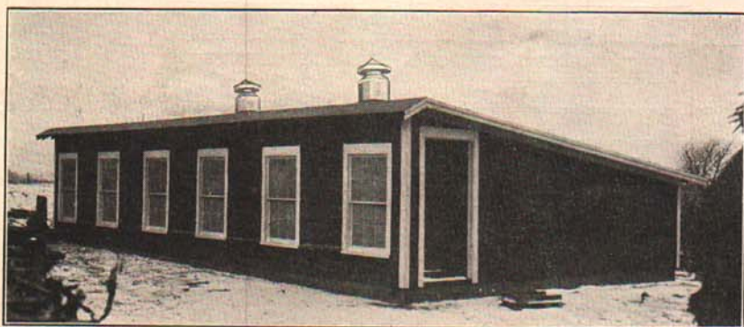
Fig. 1.—The Michigan Shed Type Poultry House—an efficient house of simple and economical design.
