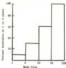
Fig. 2 — The relative availability of ground limestone as influenced by mesh size.
