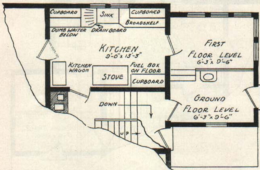
Fig. 5. This is the same kitchen as that of Fig. 2, with a larger men's washroom at ground level and a porch enclosed with windows. Meals may be served here, or it may be used as a laundry room.
