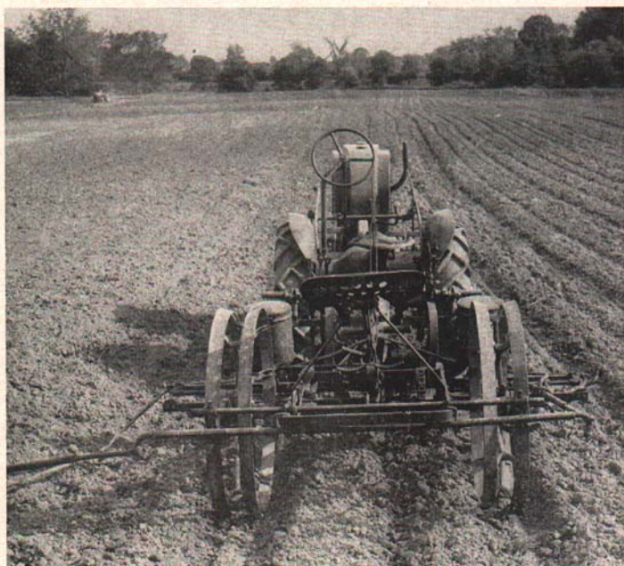
Fig. 14. Soybeans are being wheel-track planted, June 4, on land which has just been plowed with a revolving bladed tiller attached to the plow. The row width is 36 inches with 28-inch "guess" rows. Note the nice condition of the soil. Soil moisture was good, germination was fast and uniform. This method of planting has worked very well for corn, giving quick germination and good stands.
