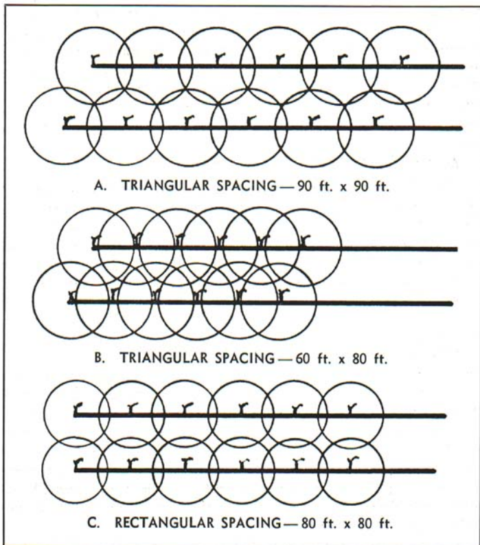
Fig. 2. Effect of sprinkler spacing and arrangement on the application of water for frost protection. Sprinklers in Arrangements A and B represent a 110-foot diameter of coverage. Those in Arrangement C represent a 95-foot diameter of coverage.
