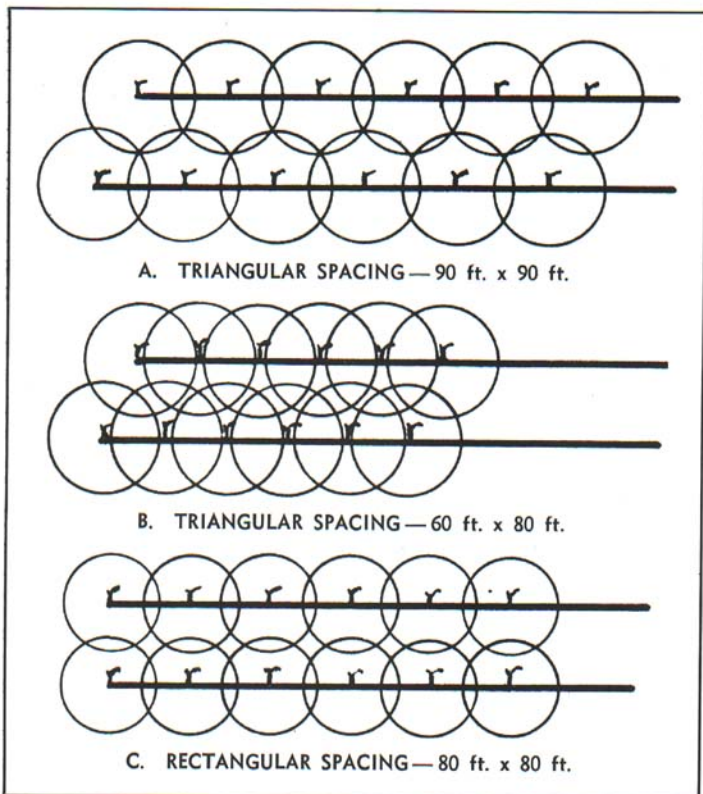
Fig. 2. Effect of sprinkler spacing and arrangement on the application of water for frost protection. Sprinklers in Arrangements A and B represent a 110-foot diameter of coverage. Those in Arrangement C represent a 95-foot diameter of coverage.
