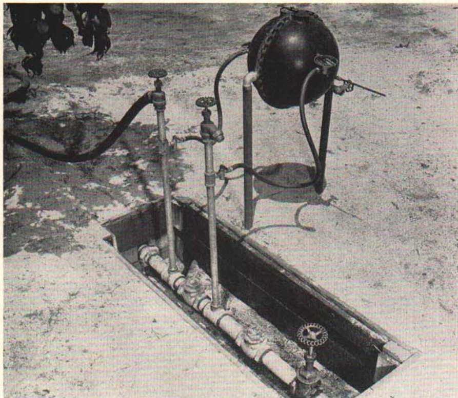
Fig. 7. Another type of commercial sprinkler-system fertilizer applicator, utilizing a pressure difference at a fitting.
