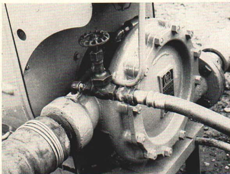
Fig. 1. Fittings used to introduce the fertilizer solution into the intake side of a centrifugal pump.
