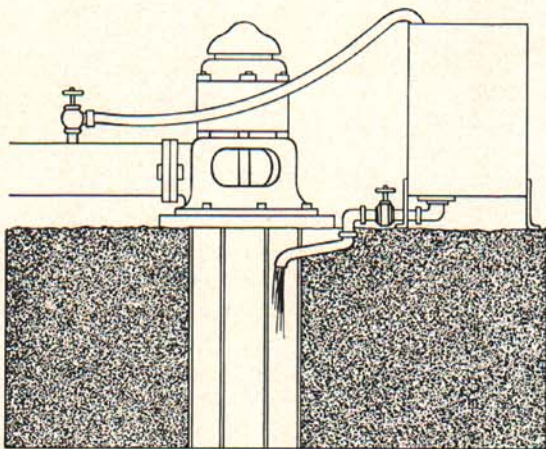
Fig. 5. One method of getting a fertilizer solution directly into a well for introduction into the irrigation system through a deep-well turbine pump. A plastic pipe could be extended to the bottom of the suction pipe of the pump.
