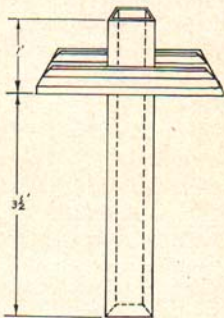
Fig. 10. Diagrammatic sketch of a "measuring well" for determination of the water level in a muck soil.
