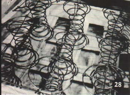
FIGURE 28. Using the center row as your guide, complete the tying of the other two lengthwise ties.
