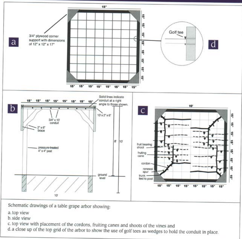
Fig. 16 – Schematic drawings of a table grape arbor showing: (a) top view; (b) side view; (c) top view with placement of the cordons, fruiting canes and shoots of the vines; and (d) a close-up of the top grid of the arbor to show the use of golf tees as wedges to hold the conduit in place.
