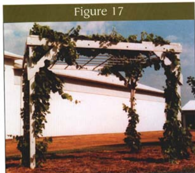
Fig. 17 – A 10-foot-square arbor for table grape production. 'Marquis' grapevines were planted in each corner and are nearing the end of their first growing season. This design can be constructed from readily available materials.
