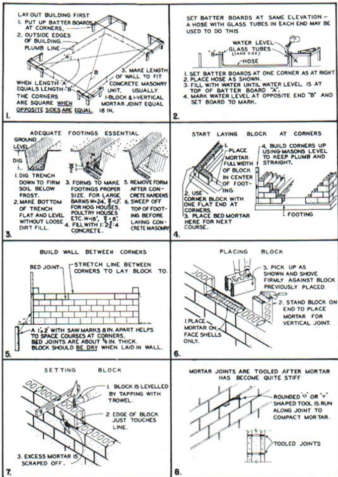
Fig. 5. Details of masonry wall construction.
