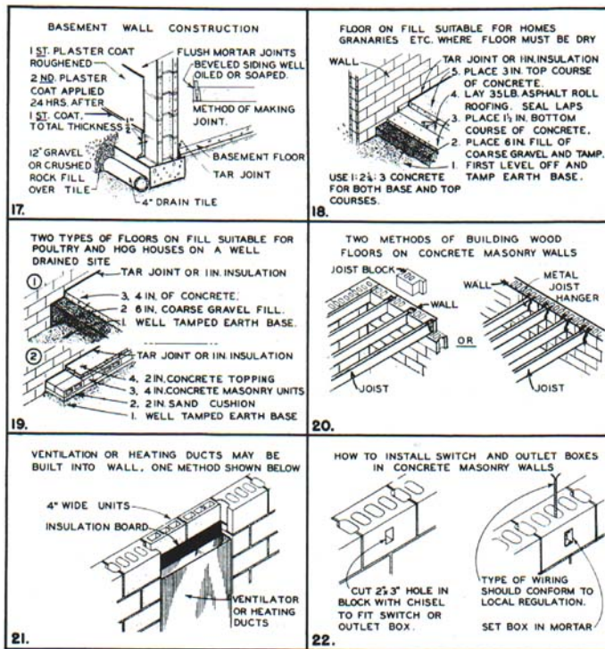
Fig. 5. Details of masonry wall construction—(Concluded).
