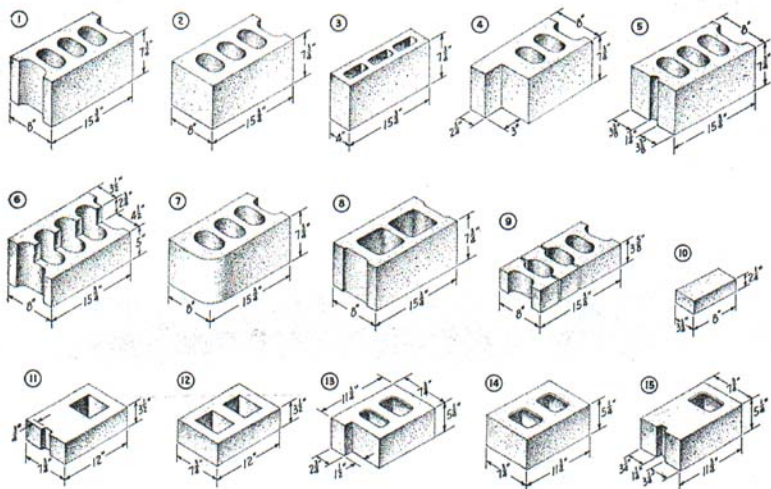
Fig. 1. Various types of concrete blocks are available for various special purposes.
