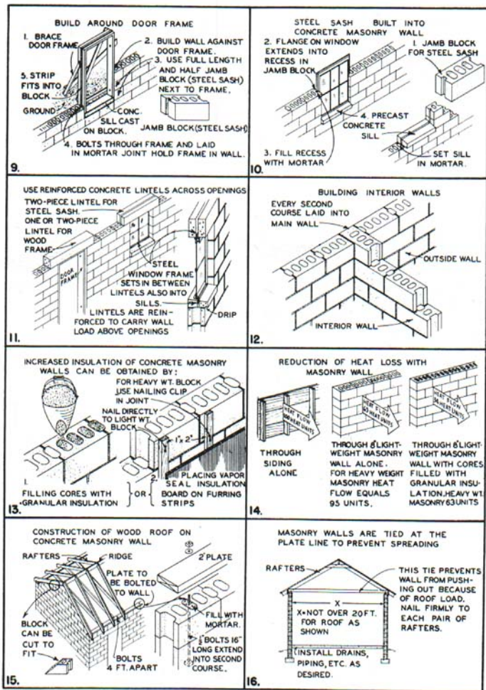
Fig. 5. Details of masonry wall construction—(Continued).
