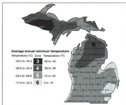
Figure 5. USDA plant hardiness zones in Michigan.
