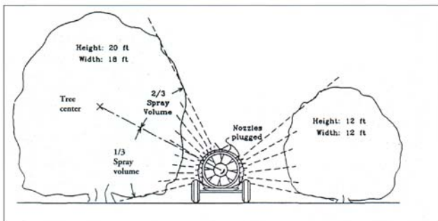
Fig. 12. Sprayer nozzling for good deposition.
