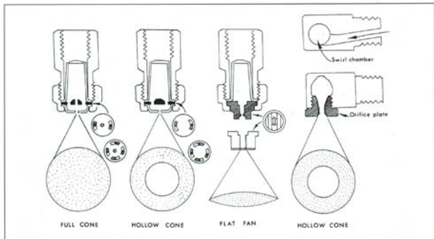
Fig. 5. Basic spray patterns.
