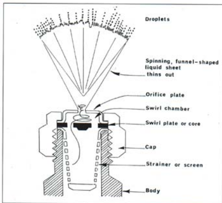
Fig. 1. Cross-section of a hollow cone nozzle.
