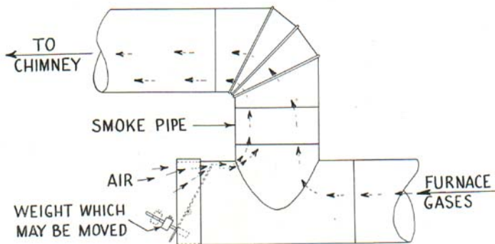
Fig. 13. Balanced damper.
