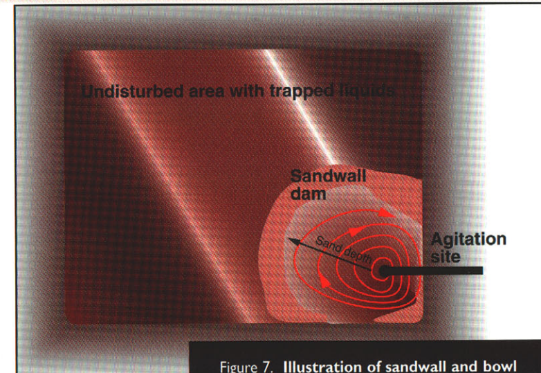
Figure 7. Illustration of sandwall and bowl formation with ineffective agitation, showing relative fluid velocity and depth of sand in a long-term storage.
