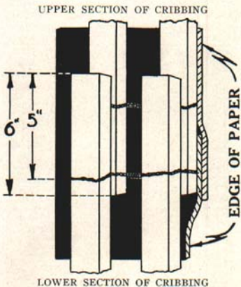
Fig. 4. A detail showing method of joining adjacent sections of cribbing and paper.
