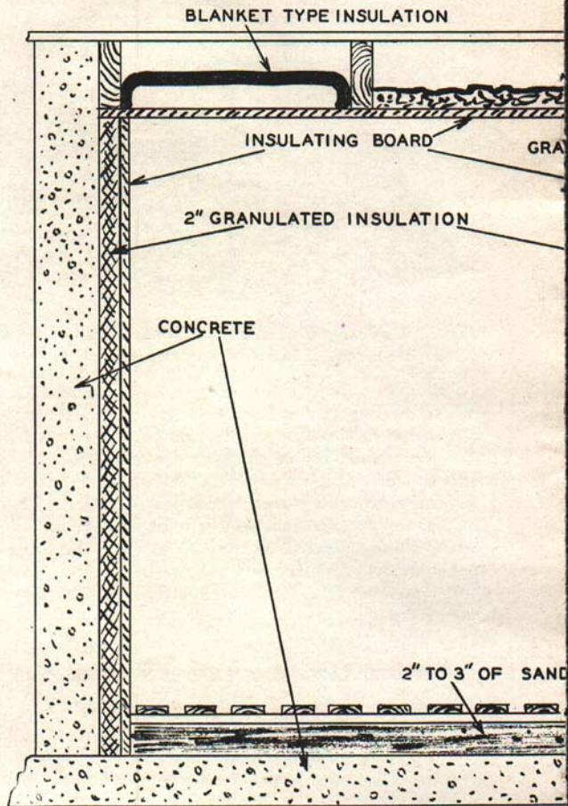
Fig. 3. Construction details for a basement vegetable storage room be insulated as illustrated. Either the blanket or fill type of insulated slatted floor will aid materially in maintaining proper moisture cond
