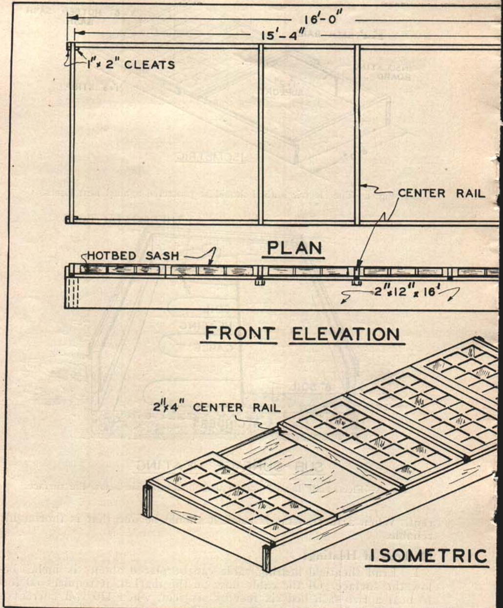
Fig. 6.—Construction details
