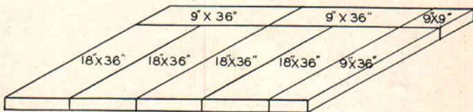
Fig. 4. Method of arranging the insulation packages for the floor of a four-can tank.
