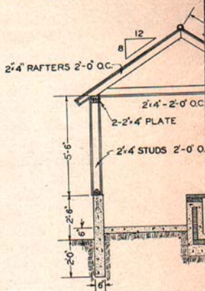
SECTION AA GABLE
