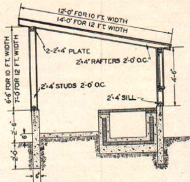
SECTION AA SHED ROOF
