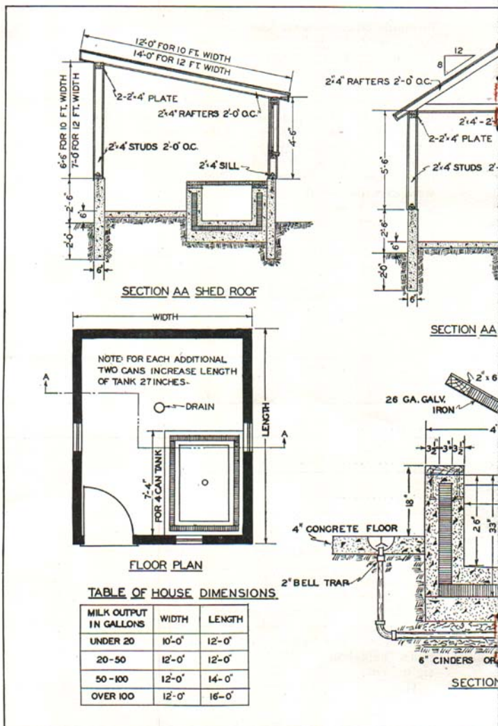
Fig. 1. Details of construction of milk house and cooling tank. (1)
