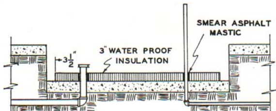
Fig. 3. Step No. 2. Here the 3" water-proof package insulation has been placed on the cement floor. Note that a 3 1/2" space is left all around the insulation for the concrete wall. The insulation should be arranged as shown in Fig. 4 (below).
