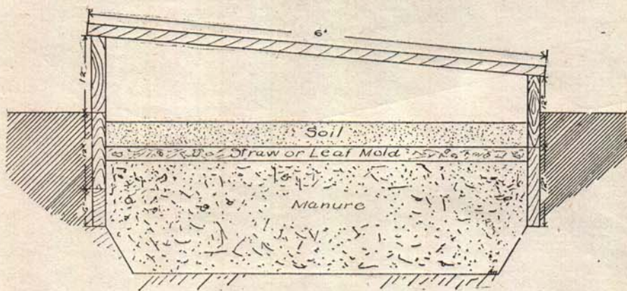
Figure 1. Crossection of a hotbed
