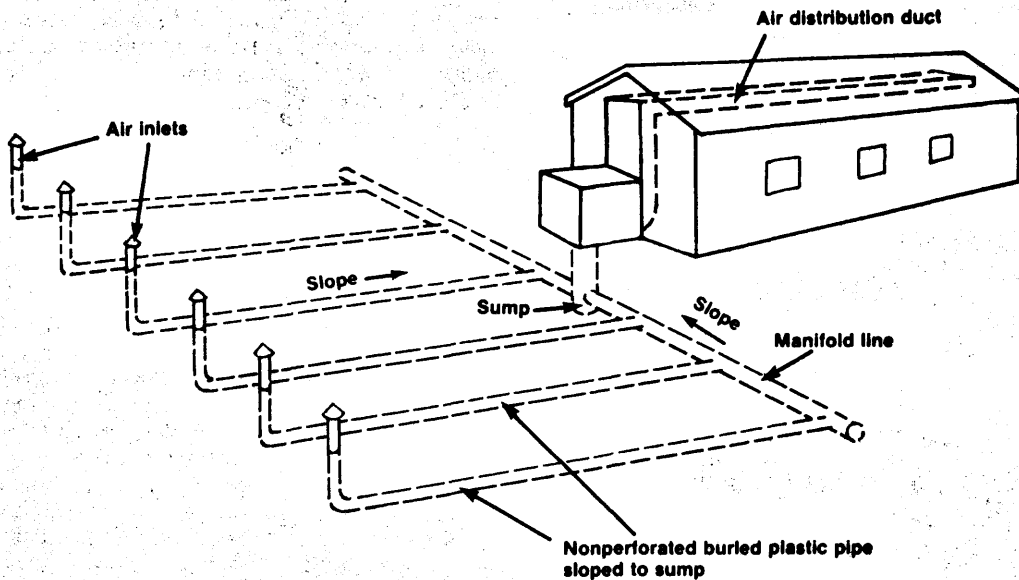
Figure 5. System layout using the lateral tubing pattern.
