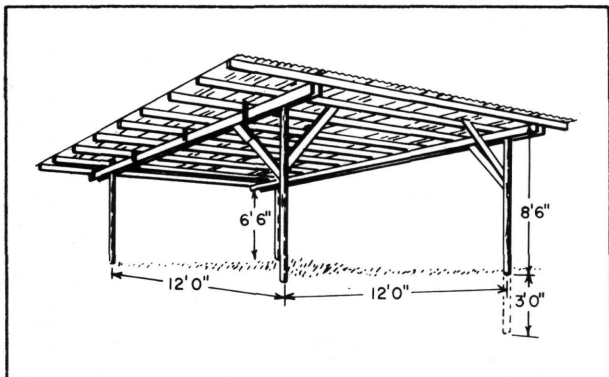
Figure 1. Shades shield out the sun's rays and provide a cool ground surface for the animals to lie on. Ideally, the high side of the shade should be located on the north to maximize radiant heat loss from the animals. See USDA Plan No. 5947 (12' x 16' shade) and No. 6257 (16' x 16' shade) available from the Agricultural Engineering Department at your state Land Grant University.
