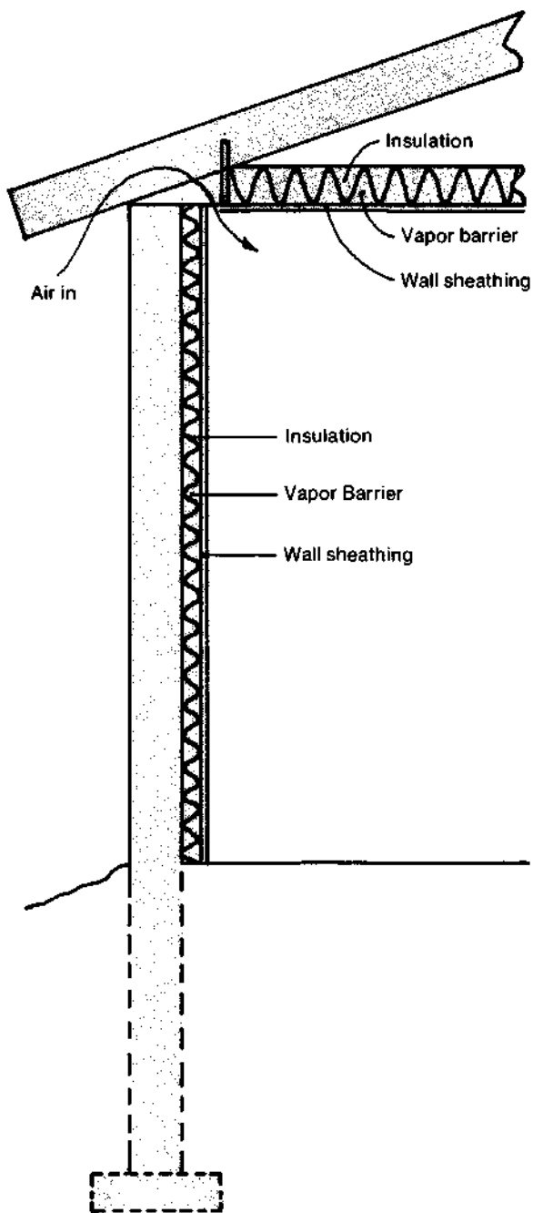
Fig. 10—Typical insulation placement.
